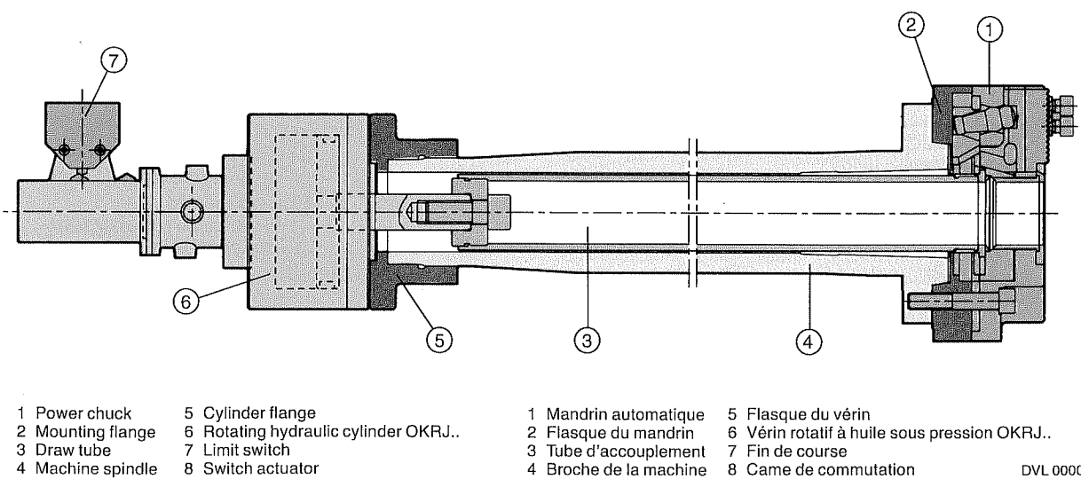
Fig. 2 ▲ shows an example of "partial open centre" chucking; the hydraulic cylinder and the chuck are connected by a draw tube. This makes it possible to carry out a limited extent of bar work. The draw tube must be balanced dynamically in two planes; the maximum permissible residual imbalance is 5 g at the outer diameter in each plane. The draw tube dimensions must be adequate for the force transmitted.
