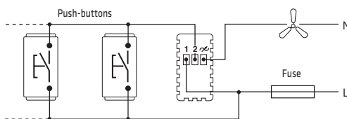
Command and adjustment from several points with NO push-buttons
